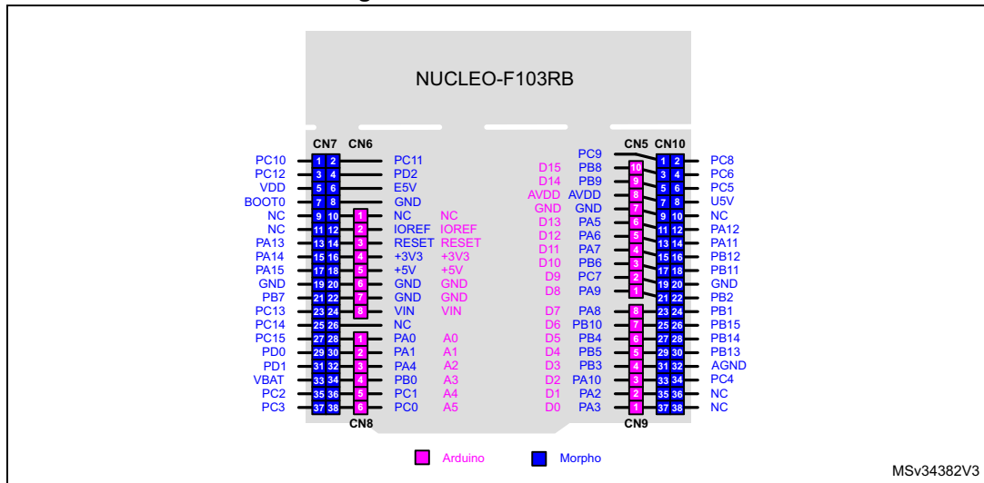
Figure 13. NUCLEO-F103RB
